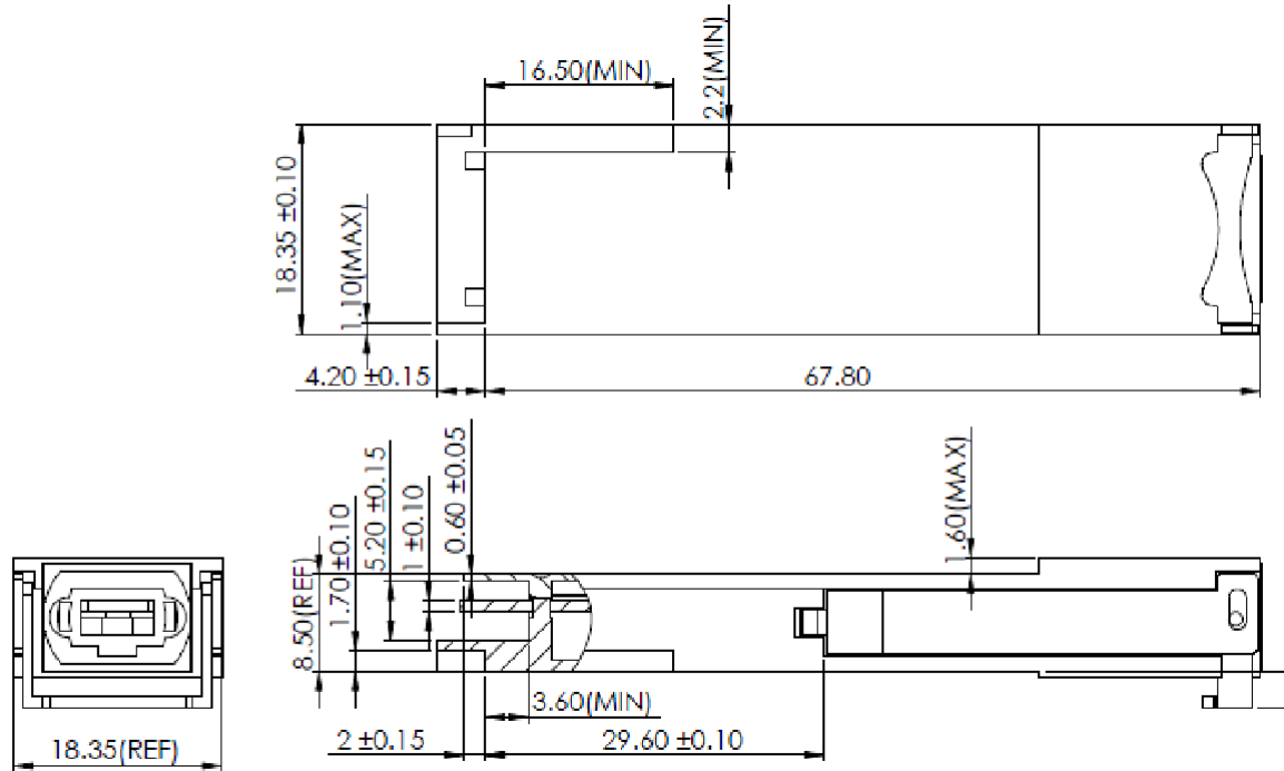
40G-Q-LR4
